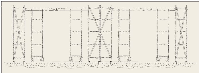
Double-Length System
